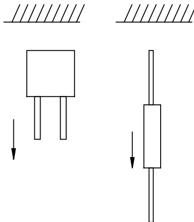
FIGURE C-1. Lead-pull direction .
