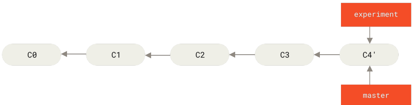
Figure 38. master 分支的快进合并
