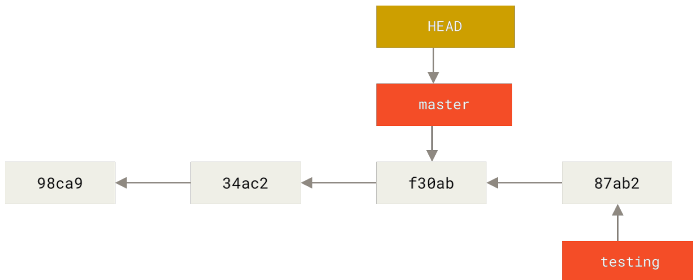
Figure 16. 检出时 HEAD 随之移动
