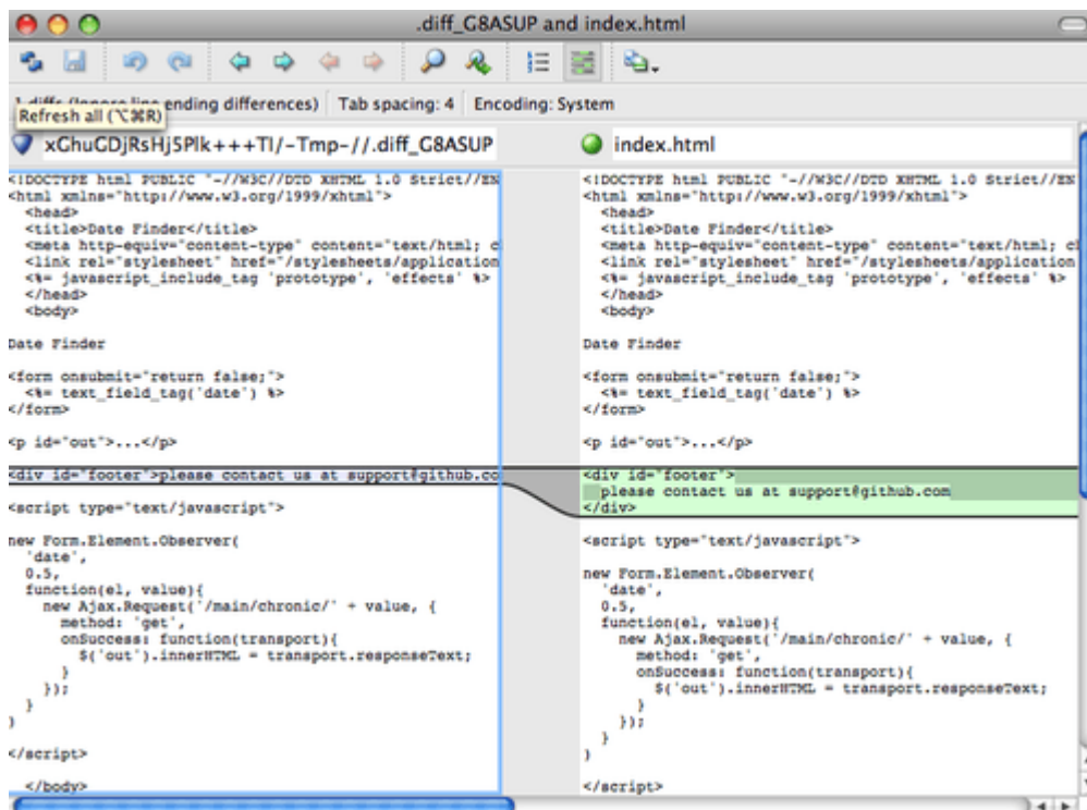
Figure 143. P4Merge.
